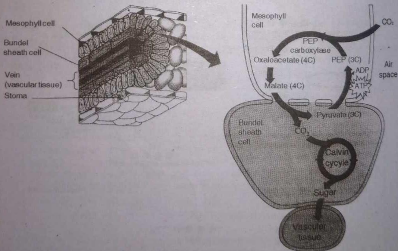
Fig.11.6 The \text{C}_4 anatomy and pathway
